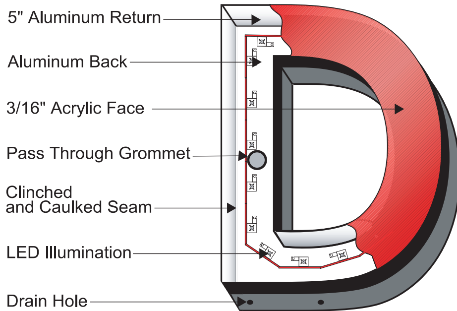
FRONT VIEW
